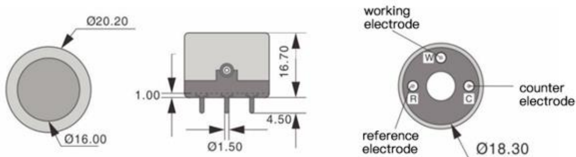
Figure 2.1. Mechanical dimension in mm
