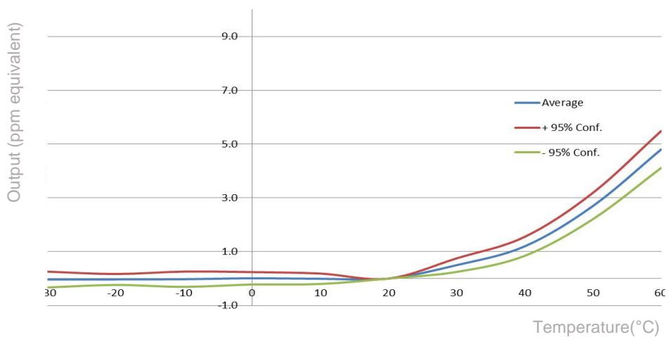
Figure 5.2. Sensor stability characteristic curve
