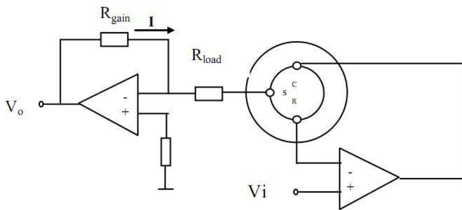
Figure 3.1. Circuits
