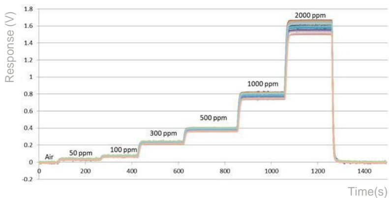
Figure 4.1. Typical sensitivity characteristic curve of the sensor
