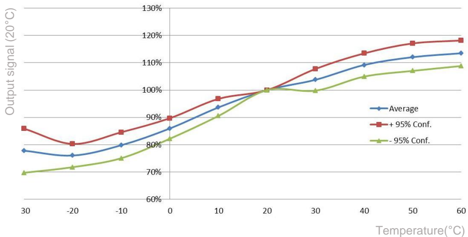
Figure 5.1. Sensor temperature and humidity characteristic curve
