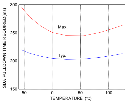
Figure 5.7. SDA pull down time
