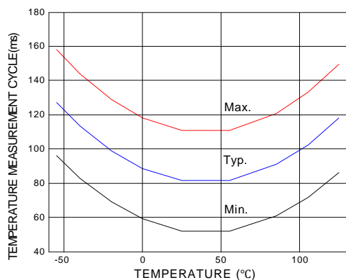
Figure 5.5. Temperature measurement cycle
