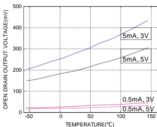
Figure 5.3. Open drain output voltage
