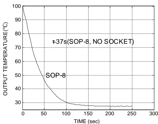
Figure 5.4. Thermal response time
