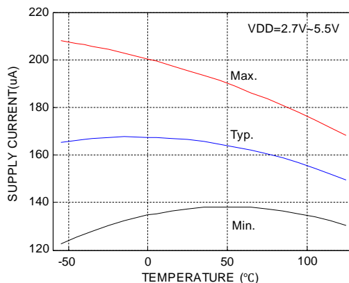
Figure 5.6. Supply current
