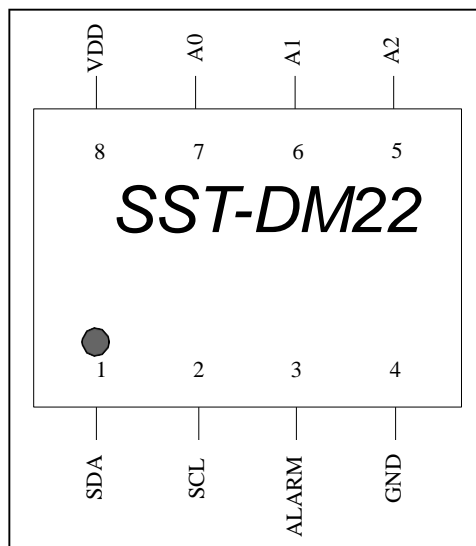
Figure 1.1. Pin out diagram
