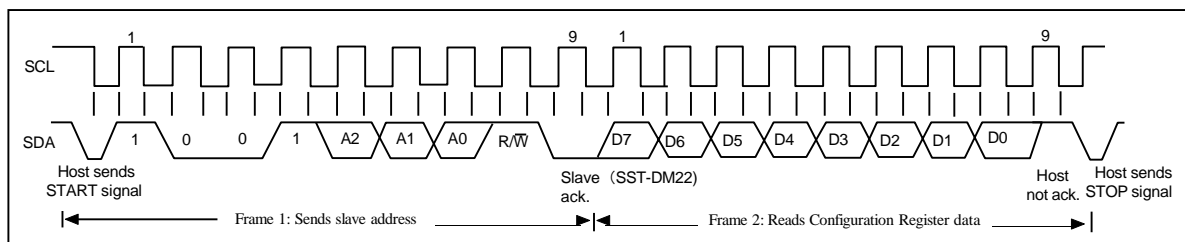
Figure 2.7.1. Read data from the Configuration Register
