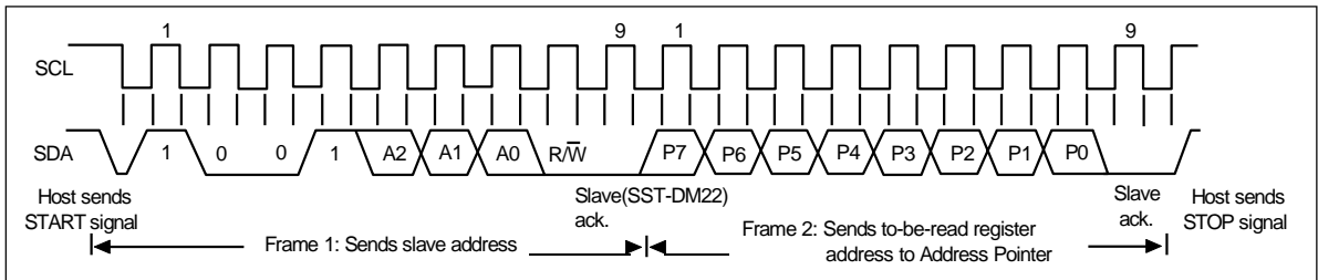
Figure 2.6.1. Write to the Address Pointer Register to select the register for subsequent operation
