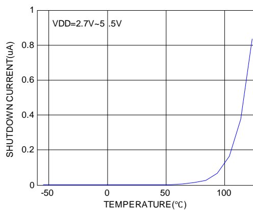
Figure 5.8. VDD current at shutdown
