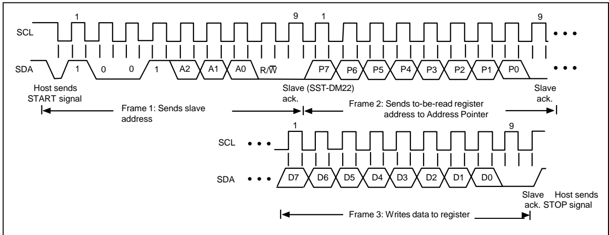
Figure 2.6.2. Write to the Address Pointer Register and then write the single byte data to the 8 bits register
