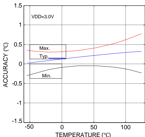
Figure 5.1. Temperature accuracy at 3V
