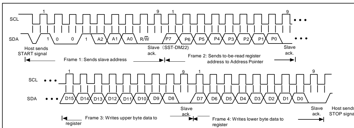
Figure 2.6.3. Write to the Address Pointer Register and then write the double byte data to the 16 bits register
