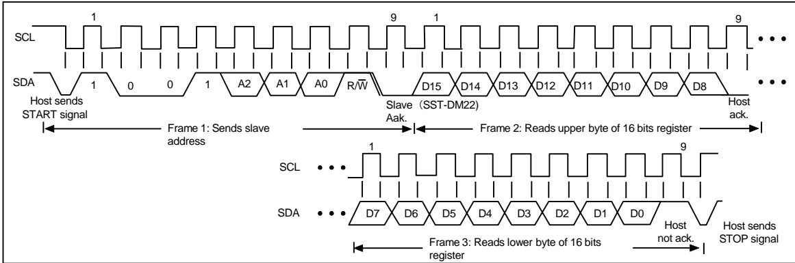
Figure 2.7.2. Read data from a 16 bits register
