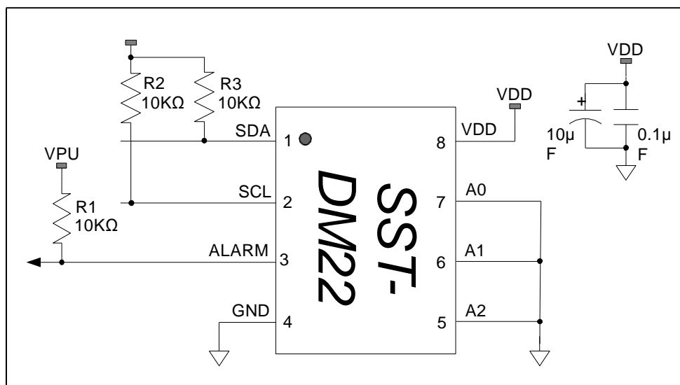
Figure 3.1. Typical application diagram
