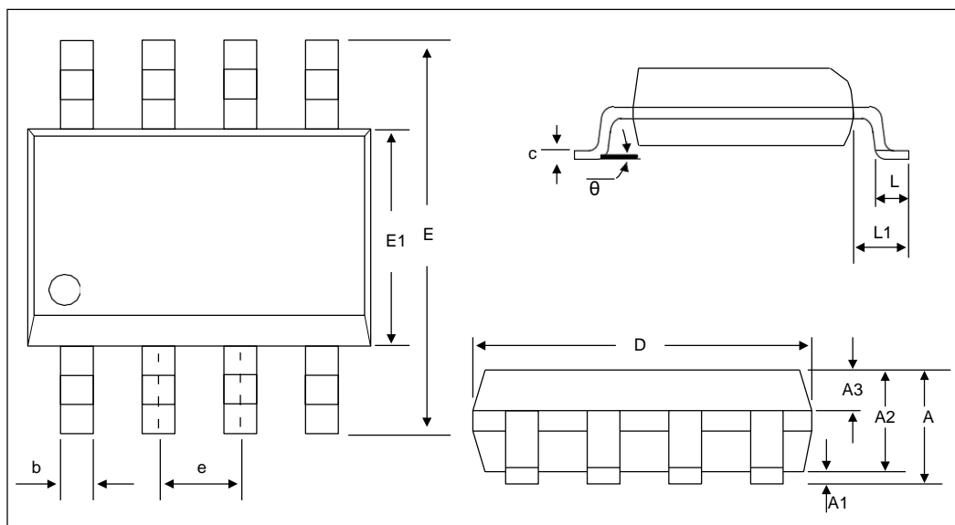
Figure 6.1. Dimension housing pack
