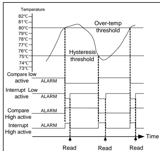
Figure 2.3. ALARM responses to temperature
