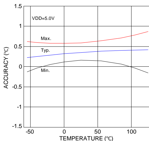
Figure 5.2. Temperature accuracy at 5V
