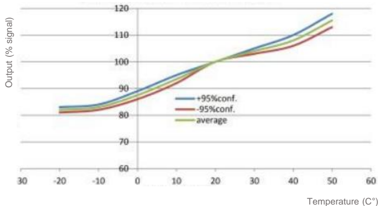
Figure 4.1. Sensor temperature and humidity characteristic curve
